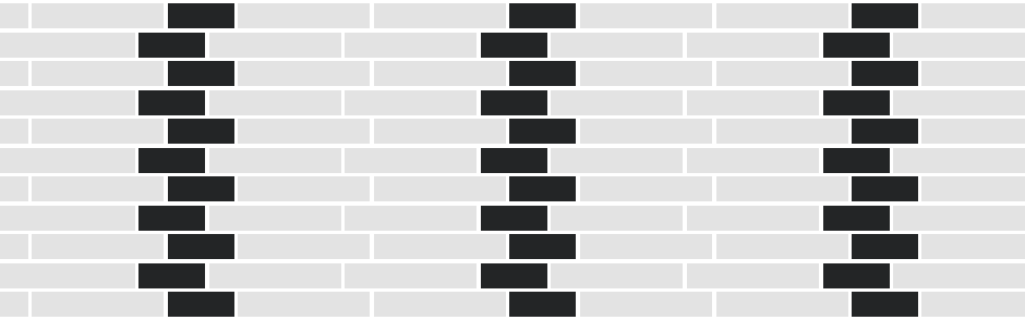
Silesian bond
