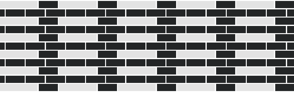
Dutch bond
